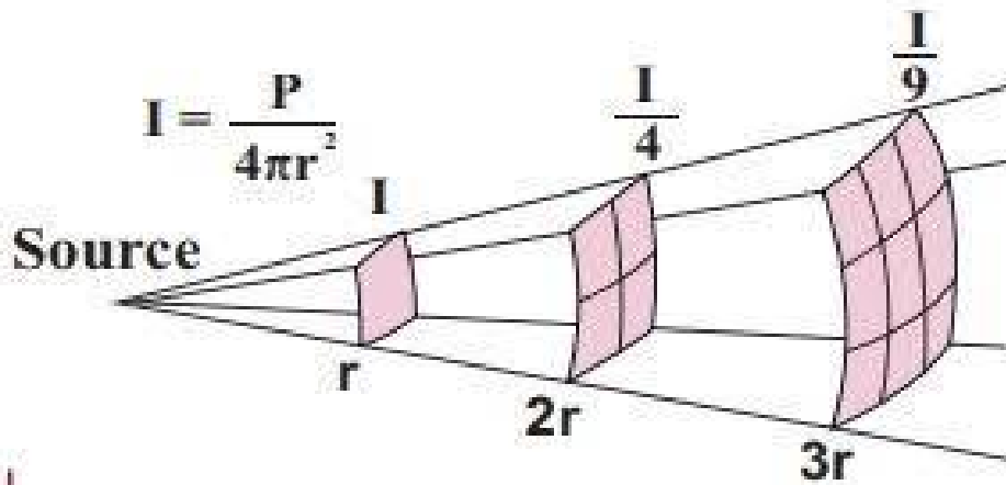
Figure 11.35 Intensity of sound waves
