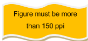
Figure 1. Formatting rules
