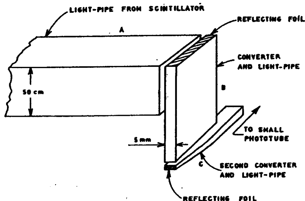
FIG. 1. Light from the light-pipe or scintillating vat (A) strikes converter (B), in which it produces fluorescent light of slightly higher photon energy. Some of this light, being isotropic, can now be collected along the converter without further loss; and, in principle, can be used a second time to produce fluorescence in the second converter (C) to concentrate further the light onto a small phototube.
