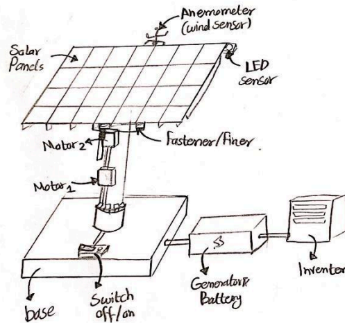
Figure 10: Sketch of dual axis solar tracker device
