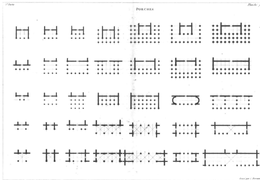
Plans for porches Jean-Nicolas-Louis Durand 1809
