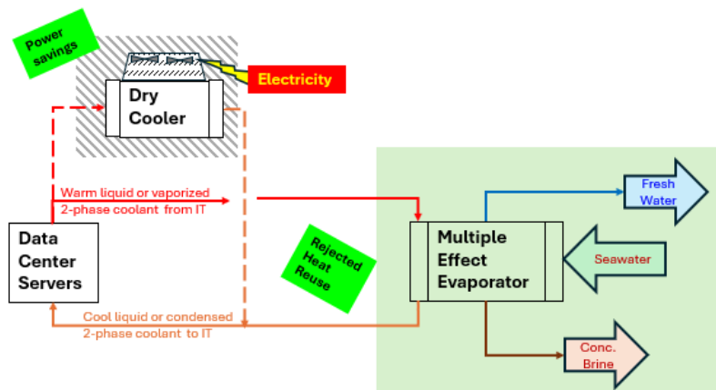
MEE Instead of Dry Cooling of TCS Coolant
