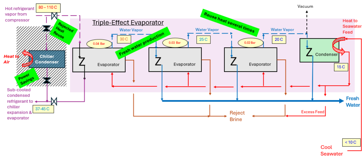
Waste heat reuse from mechanical chiller to desalinate seawater.
