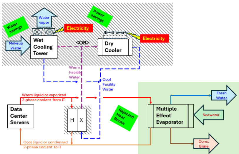
MEE Instead of Wet or Dry Cooling of Facility Water
