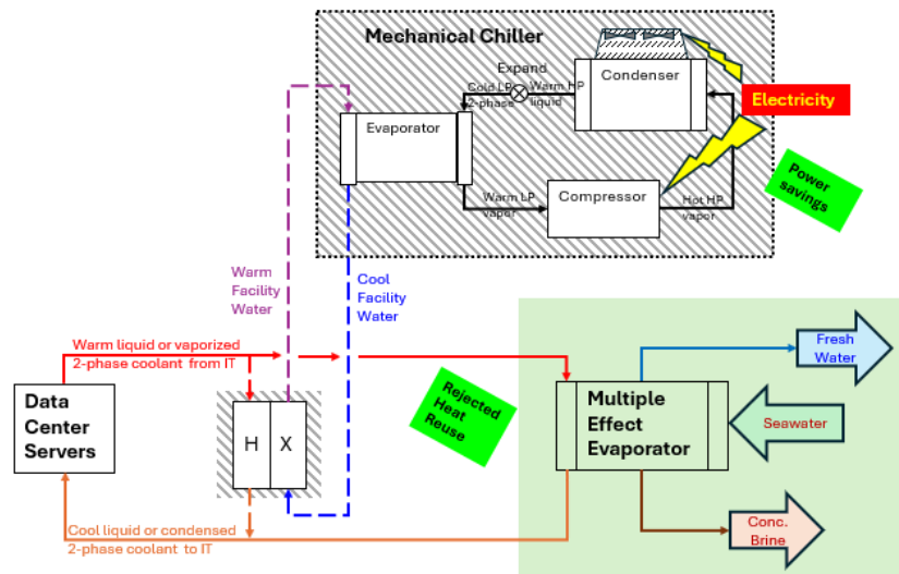
MEE Instead of Mechanical Cooling of Facility Water
