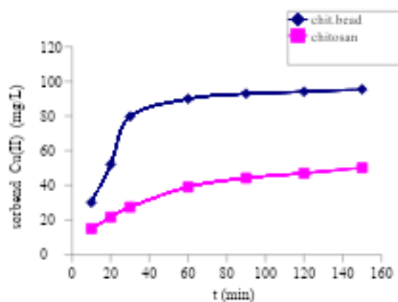
Gambar 2. Effect of contact time on the adsorption of Cu(II) on chitosan powder and chitosan beads
