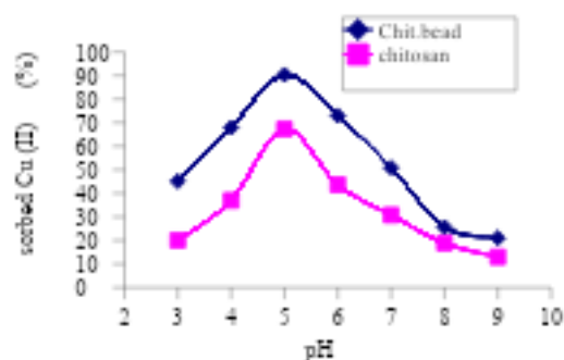
Gambar 1. Effect of medium acidity on adsorption Cu(II) on chitosan and chitosan beads
