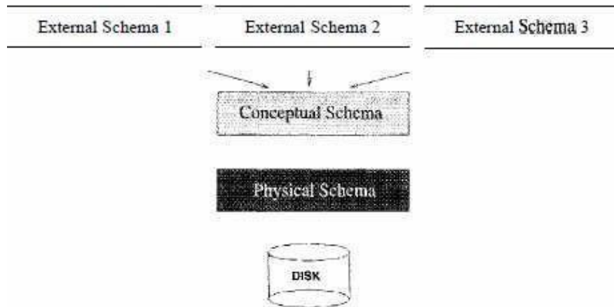
Figure 1.1: Level of Abstraction
