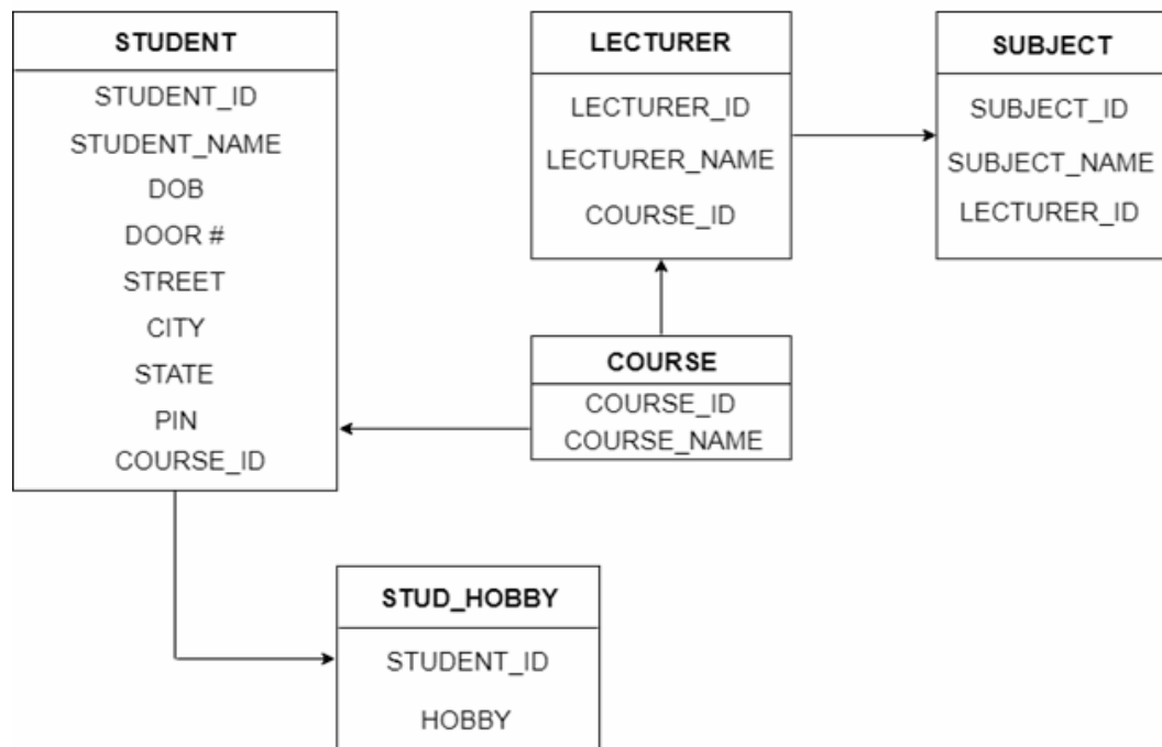
Figure 5.2: table structure of given ER diagram
