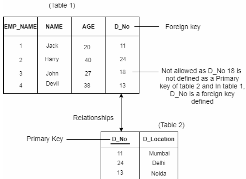
Figure 4.2: Referential integrity
