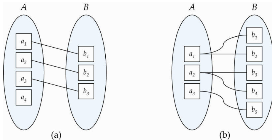
Figure 3.4: mapping cardinalities
