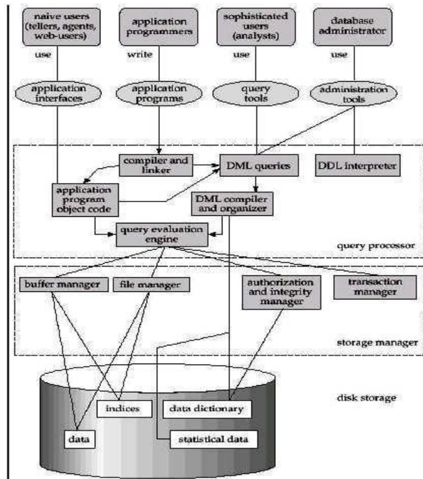
Figure 1.2: Database Architecture
