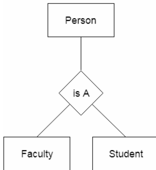
Figure 3.6: Generalization
