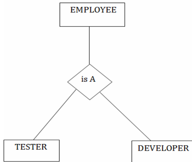
Figure 3.5: Specialization
