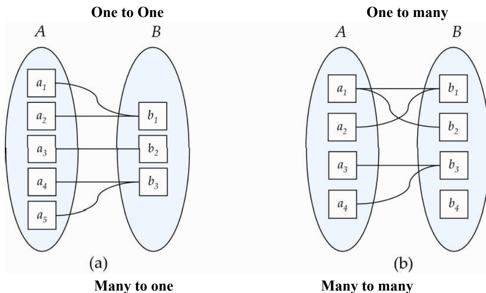
Figure 3.4: mapping cardinalities
