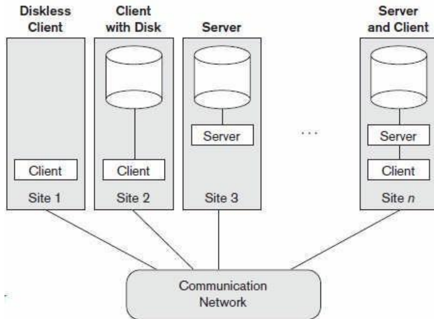
Figure 2.1: Client/Server architecture
