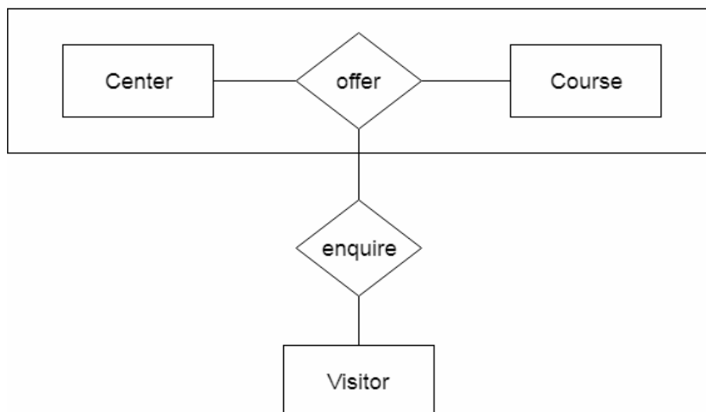
Figure 3.7: Aggregation
