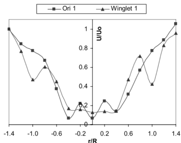
Figure 1. Axial velocity distribution behind wind turbine rotor
