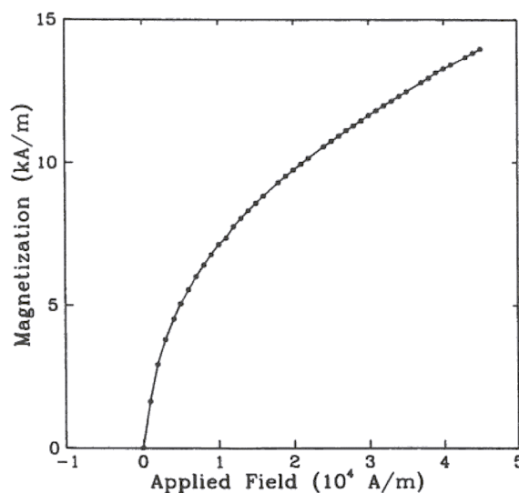
FIGURE 1. Magnetization as a function of applied field
