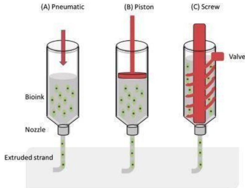
Figure: Representing extrusion based bioprinting
