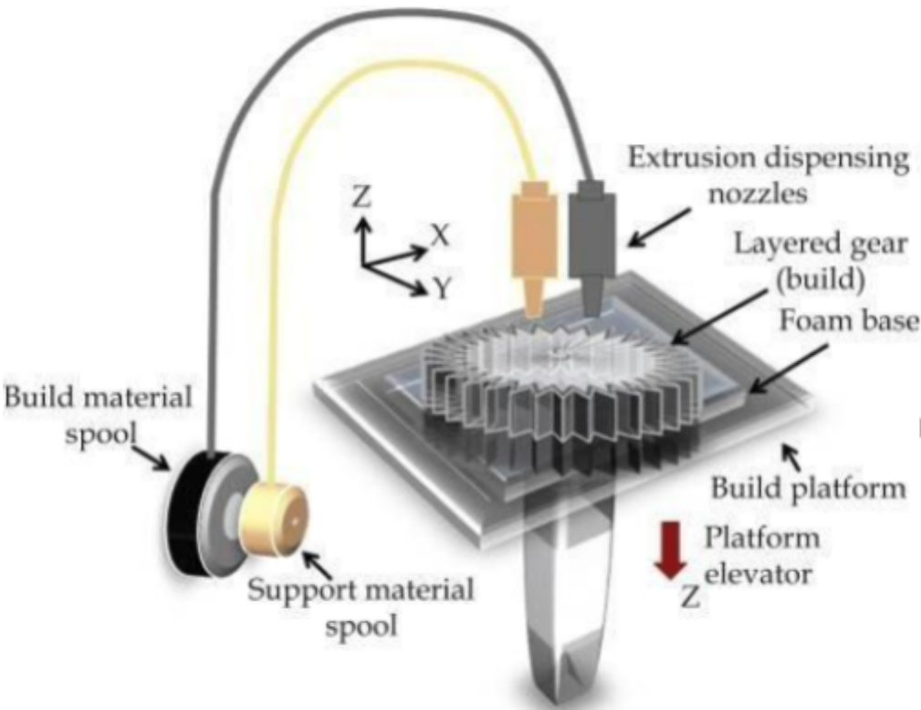
Figure: Representing fused deposition modeling
