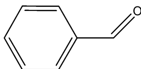
benzaldéhyde
