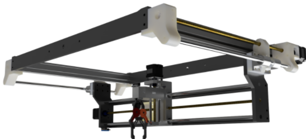
Gantry System
