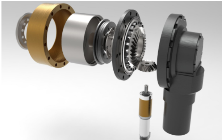
Arm Link Joints Exploded View
