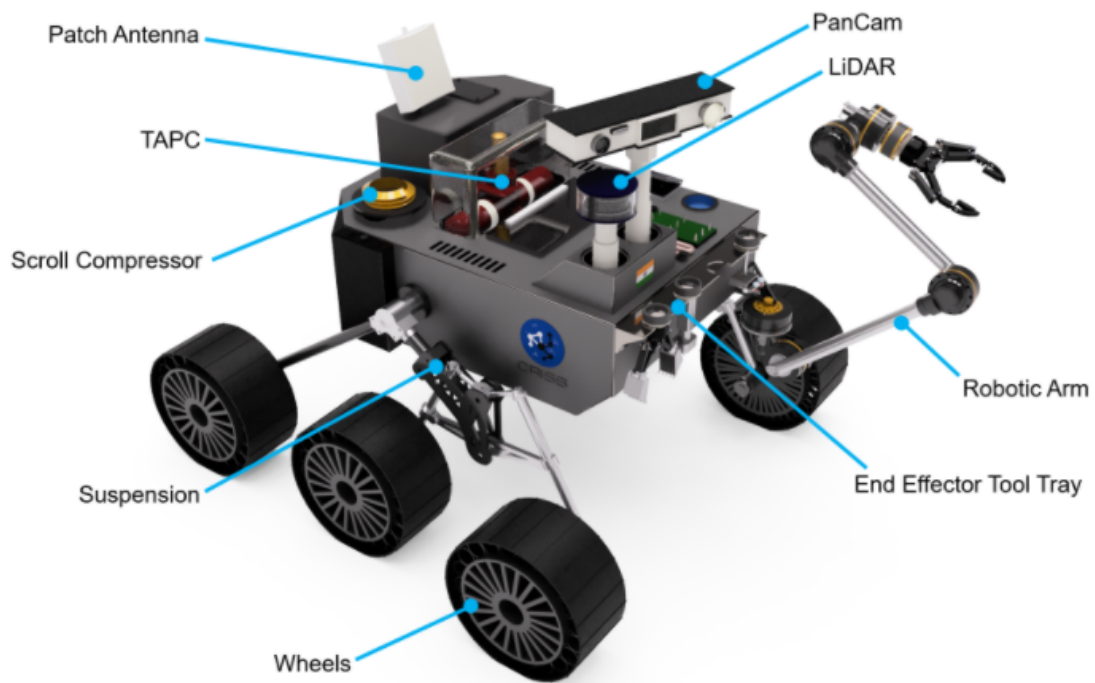
Science Rover Labelled
