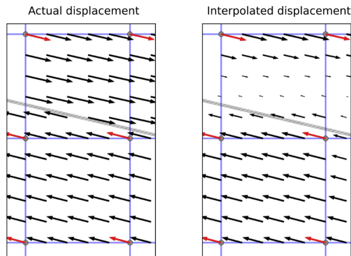
Figure B.1 — Ground displacement (left diagram) and interpolated displacement (right diagram) in a grid spanning a fault trace (hashed line).
