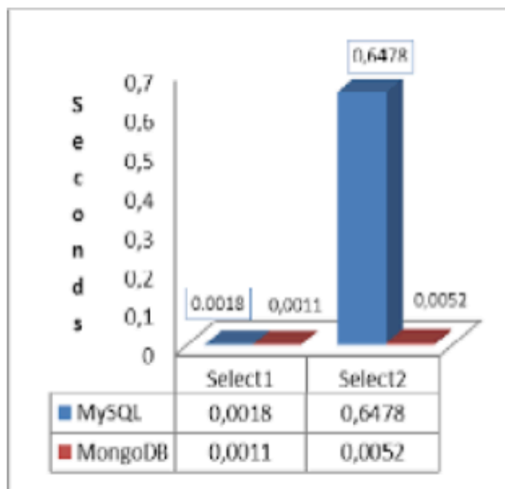
Fig. 2. MySQL vs. MongoDB select
