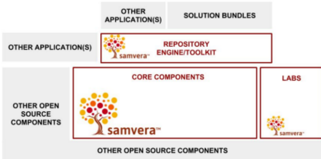
Figure one: the anatomy a Samvera application
