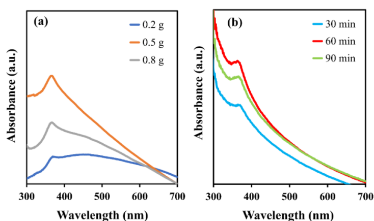
Figure 1. UV-Visible spectrum of optimization of green synthesized ZnO NPs; (a) optimization of T. catappa leaf extract (0.2, 0.5 and 0.8 g) and (b) optimization of sonication time (30, 60 and 90 min).
