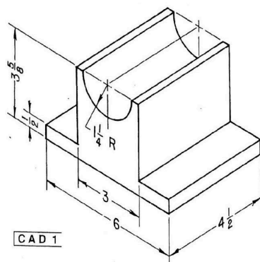
FIG. 5-61 Cradle block.
