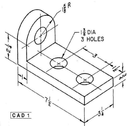
FIG. 5-63 Base.
