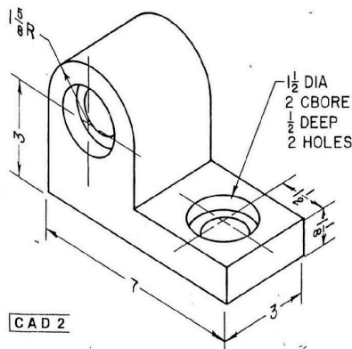
FIG. 5-64 Shaft support.
