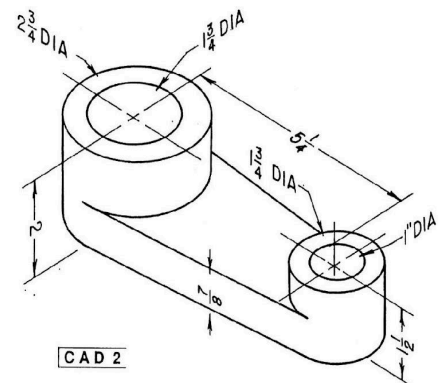
FIG. 5-66 Swivel arm.
