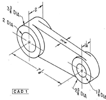
FIG. 5-62 Pivot arm.
