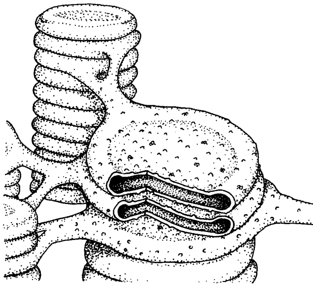
FIGURE 2-THYLAKOID
