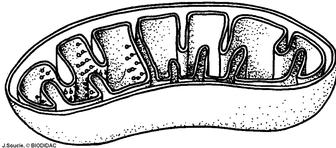
FIGURE 3 - MITOCHONDRIA Mitochondria
