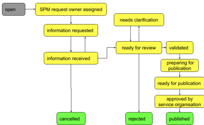
Figure 5. Onboarding workflow
