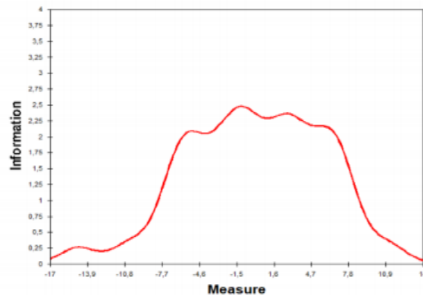
Gambar 1. Test Information Function
