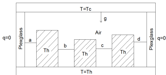
Figure 1. Cavity geometry
