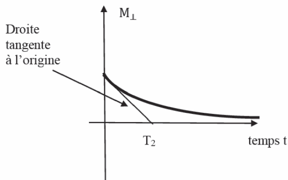
Figure 3 - Relaxation transversale
