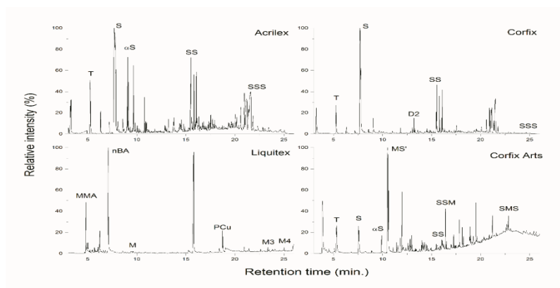
Fig. 4. Py-GC/MS spectra of phthalo blue (BPc) paints: Acrilux, Corfix, Corfix Arts (BRA) and Liquitex (USA)
