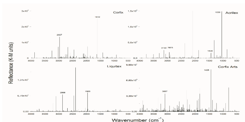
Fig. 1. FTIR spectra of phthalo blue (BPc) paints: Acrilex, Corfix, Corfix Arts (BRA) and Liquitex (USA)
