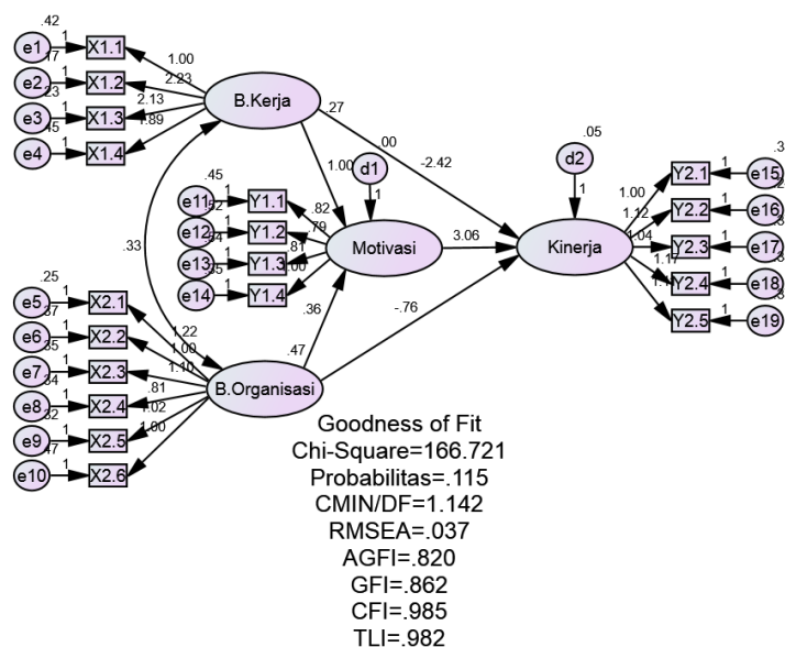
Gambar 1. Full Structure Model SEM
