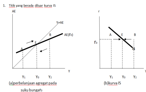
Gambar 1. Kurva IS
