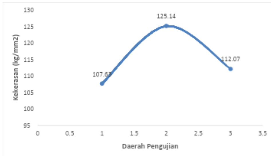
GAMBAR 2. DISTRIBUSI KEKERASAN
