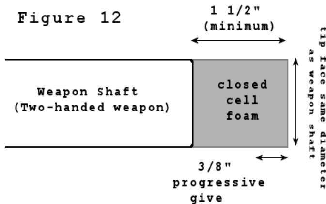
Figure 12 - Two-handed Rattan weapons up to 7.5 ft in length Thrusting Tip Construction-
