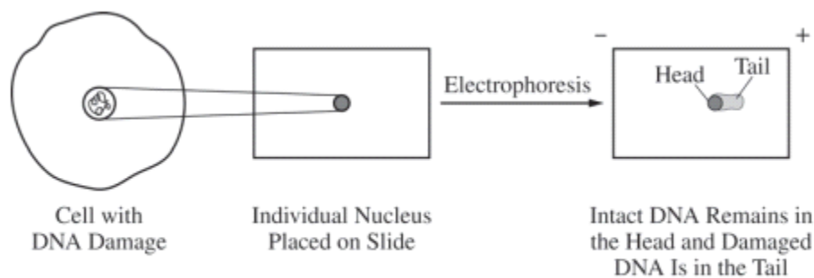
Figure 1. Comet assay to detect double-stranded breaks in DNA
