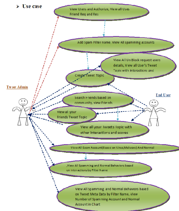
Fig 5.4: Use case Diagram
