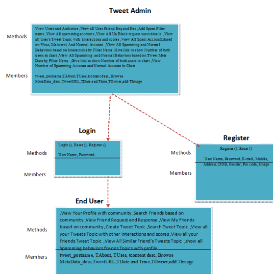
Fig 5.5: Class diagram
