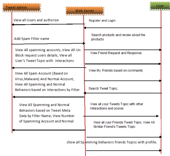
Fig 5.6: Sequence diagram
