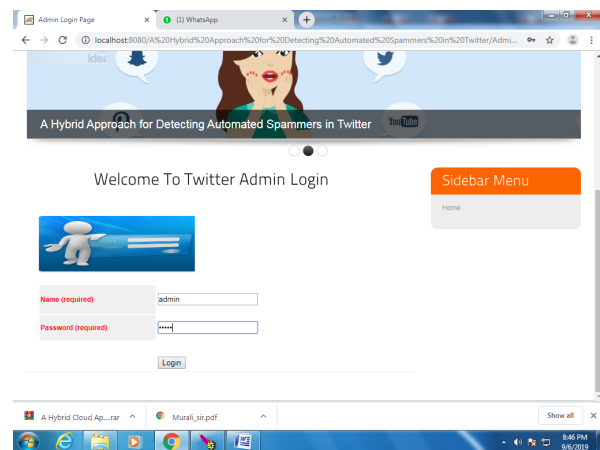
Fig 6.2: Admin Page
