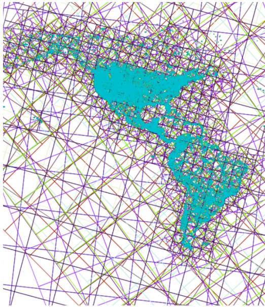
Figure 2. QuadTree implementation
