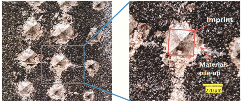
Fig. 3. Optical images of Marcellus shale taken by Echo Revolve optical microscope, indentation grid is parallel to the bedding direction. Left: the grid of the indentation imprints grid, right: zoom in to a single imprint.
