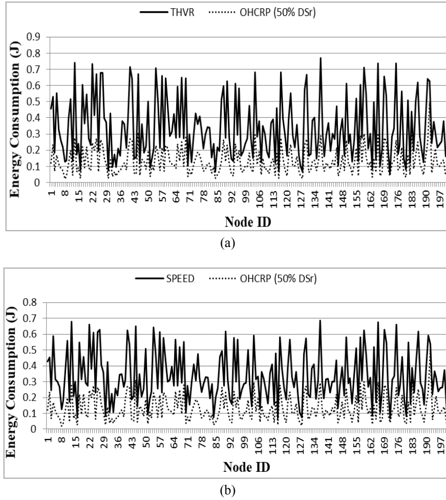
Figure 2. Nodes energy consumption in network (a) OHCRP (50% DSr) vs SPEED and (b) OHCRP (50% DSr) vs THVR
