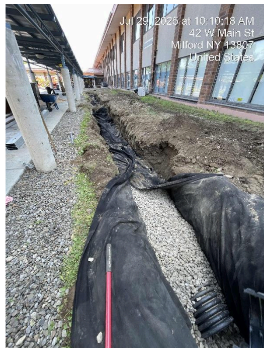
Main Campus Drainage Install
