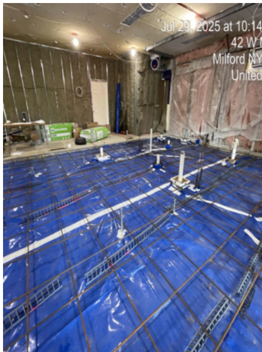
Kitchen, Under-Slab Utilities Installed
