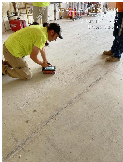
Science Room Floor Scanning
