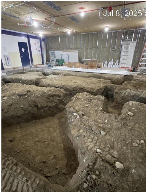
Excavation for Under-Slab Utilities, Kitchen
