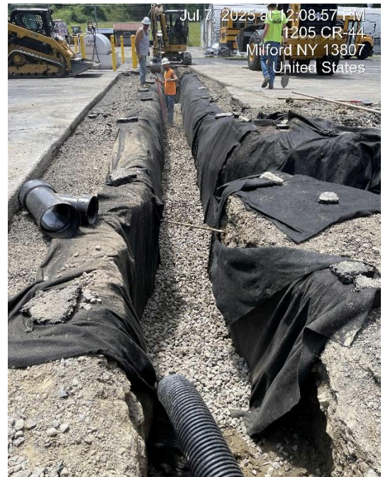
Site Drainage Install, Bus Garage
