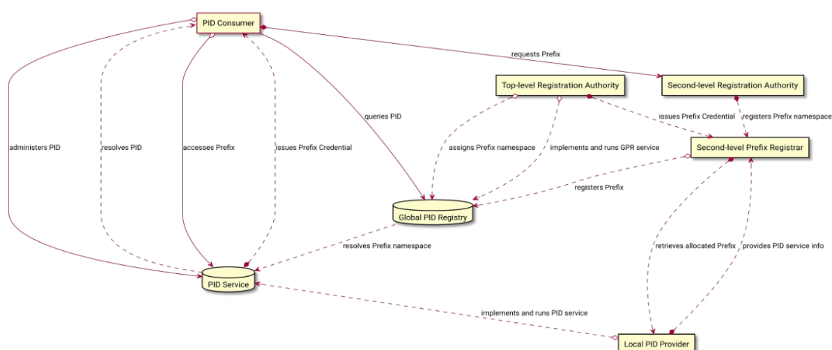
Figure 1. Centralised PID Administration and Implementation Schema
