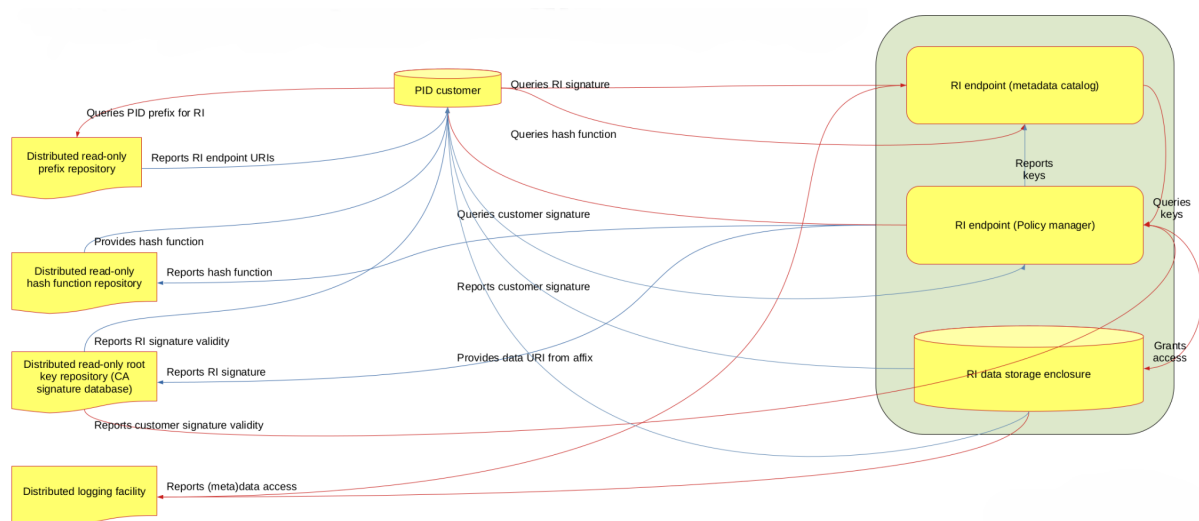
Figure 2. One of the Possible Decentralised PID Workflow Implementation Schemas
