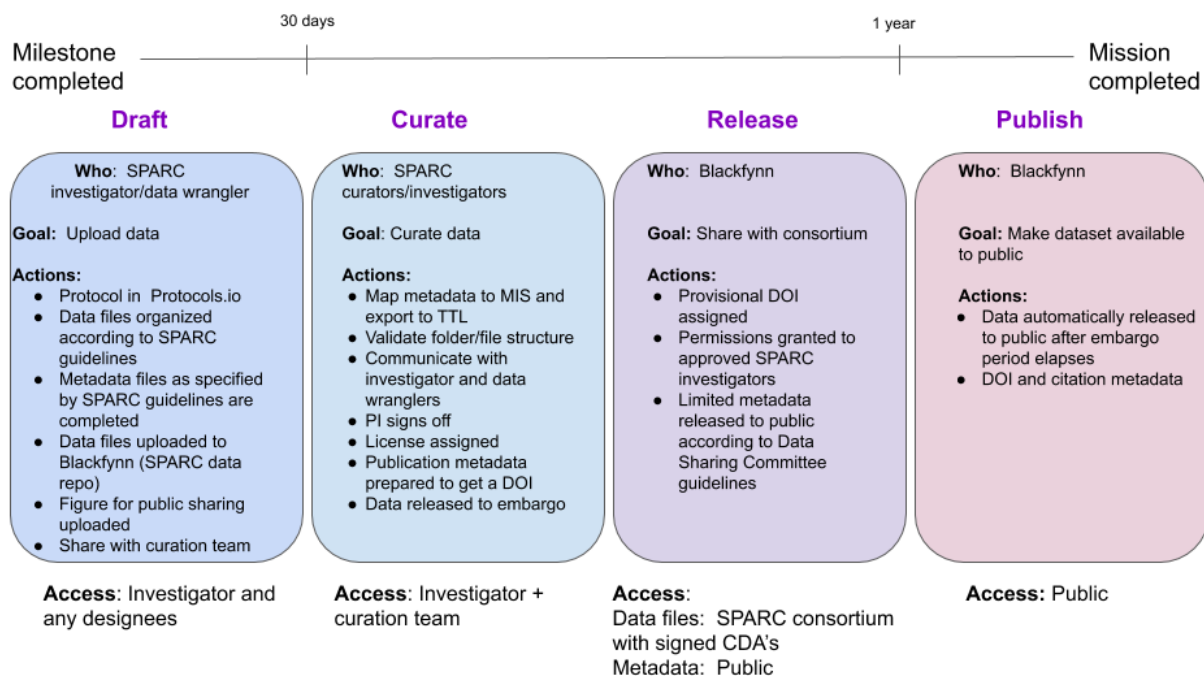
Figure 12: Overview of the entire submission-curation-publishing workflow
