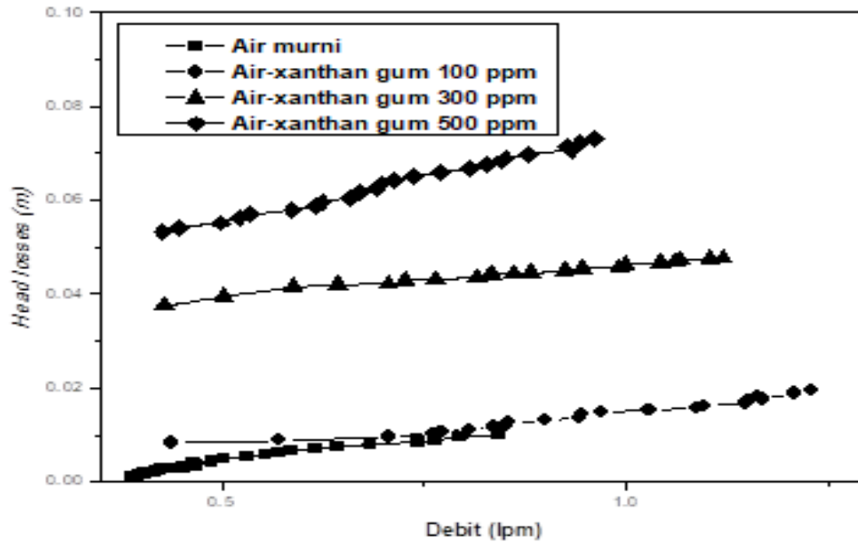
Figure 3. Comparison of the discharge value to the pressure drop value
