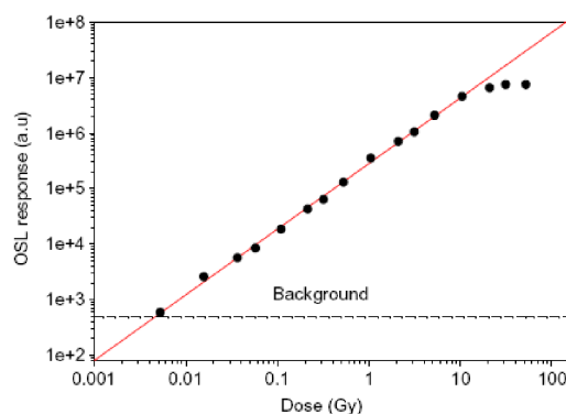
Figure 1. OSL vs. administered dose for the studied aliquots.
