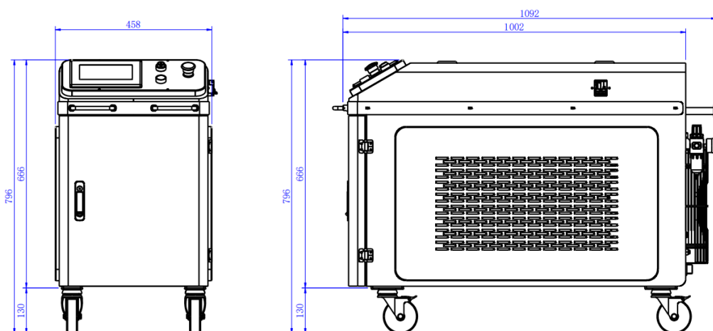
Figure 2.3 Dimensional diagram of GY-FLC1000SW laser cleaning machine
