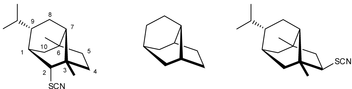
(-)-2-thiocyanatoneopupukeanane
