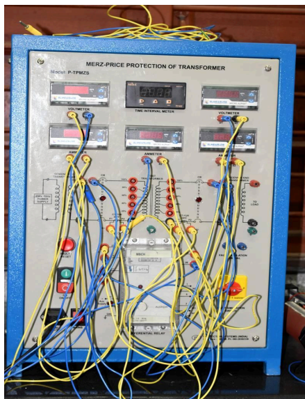
Merz Price Protection Of Transformer P-TPMZS
