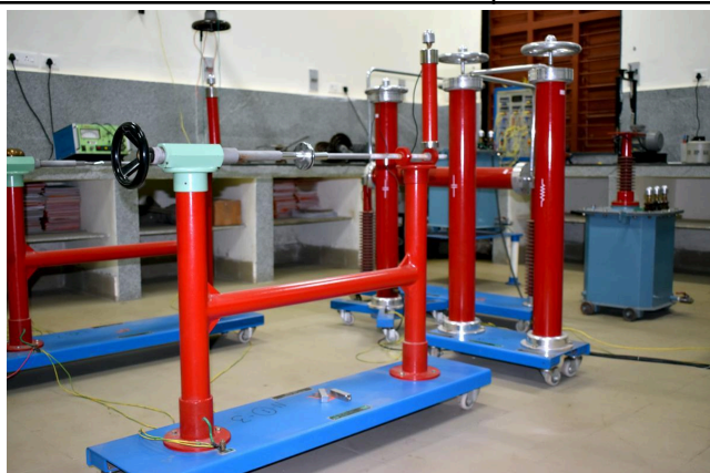
High Voltage 100kV AC DC Test Set
