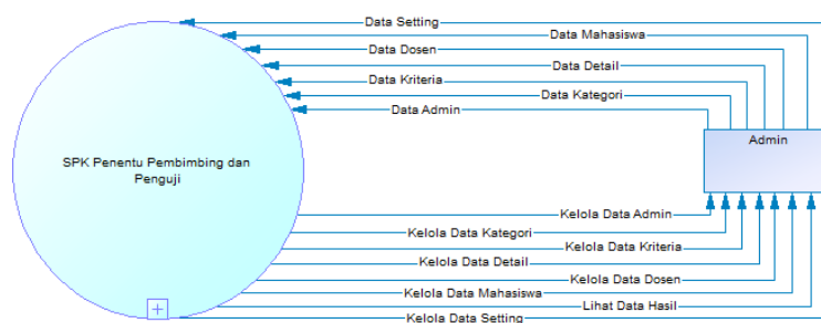
Gambar 1. Context Diagram (Book Antiqua, 11 pt)
