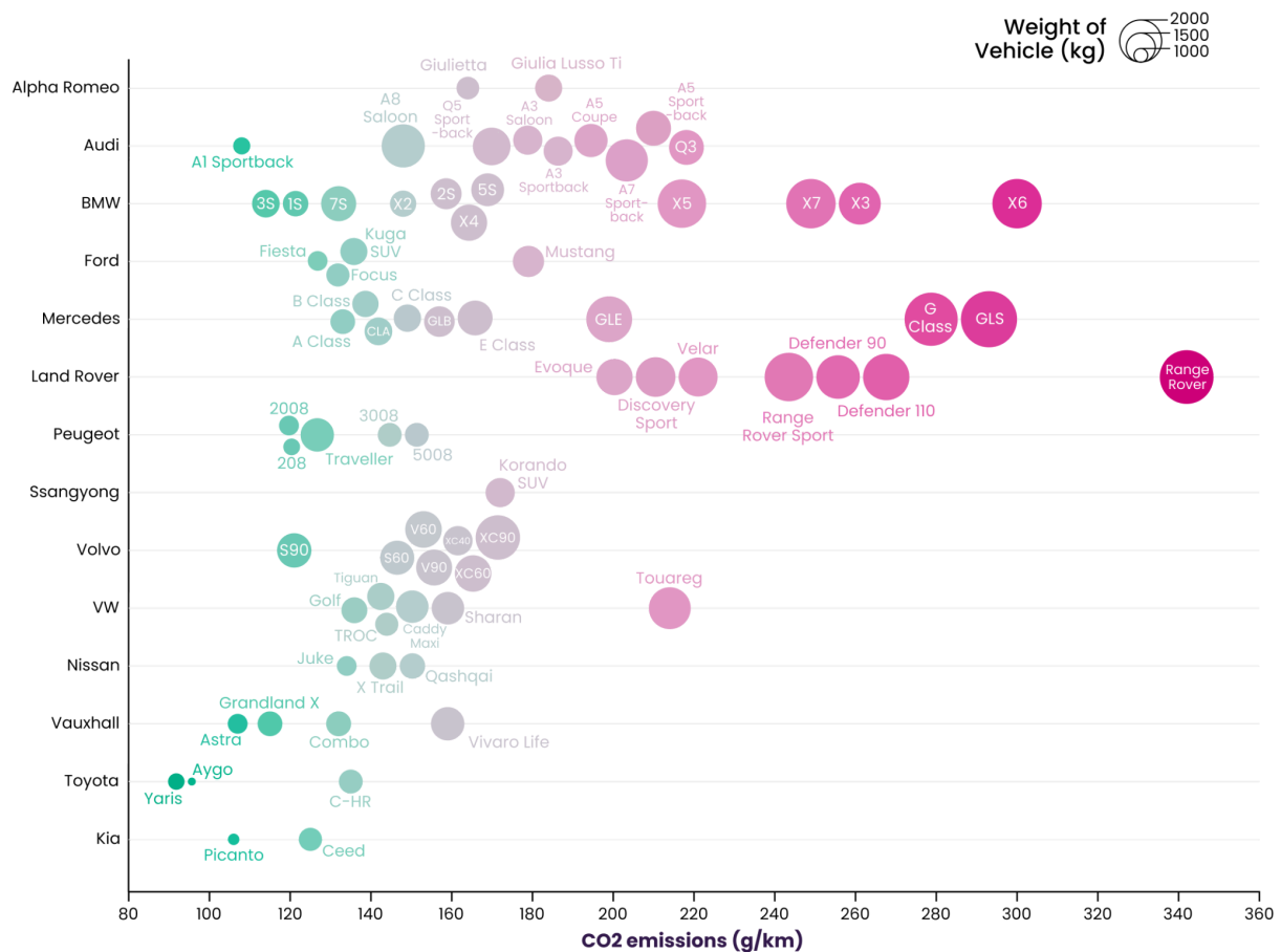
Figure 2. Heavier cars tend to have greater CO2 emissions.
