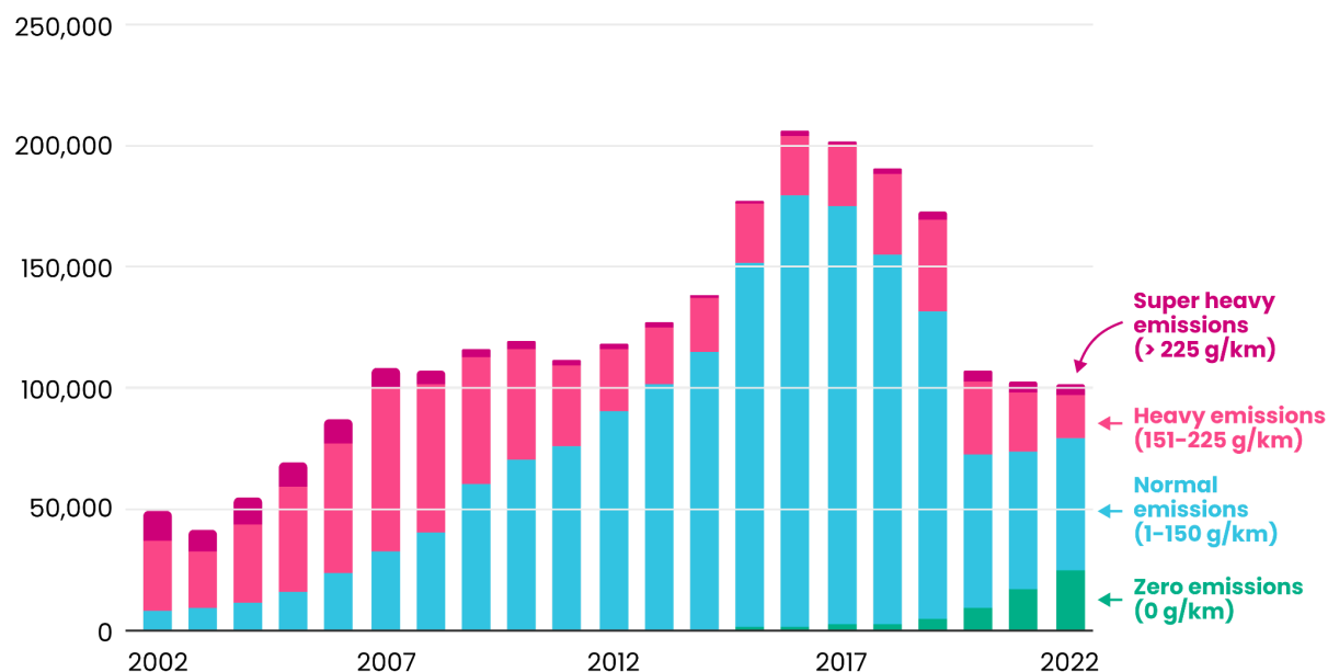
Figure 5. New car registrations by CO2 band - London.
