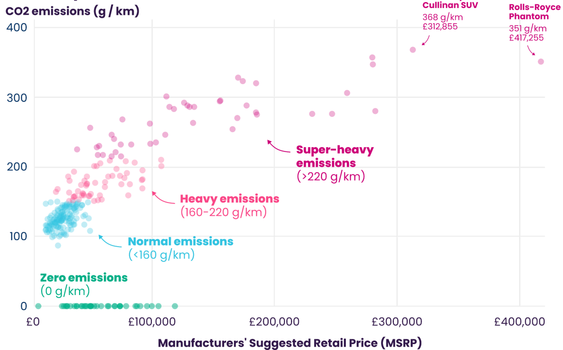
Figure 15. Price of new cars vs gCO 2 /km, UK market 2023.
