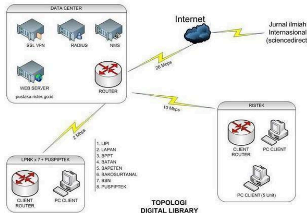
Gambar 1. Topologi jaringan digital library Pustaka Ristek
