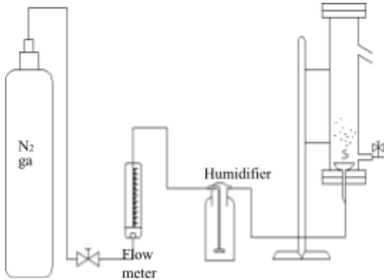
Figure 1. Flotation precipitation reactor
