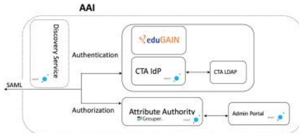
Figure: INAF-CTA AAI Architecture
