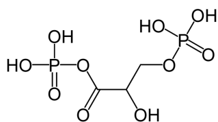
1,3-bisphosphoglycerate
