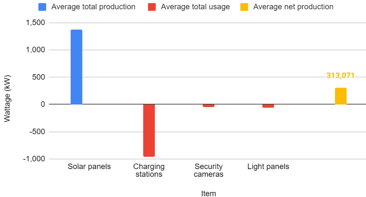
Figure 5-30: Bar graph of net solar production and usage.
