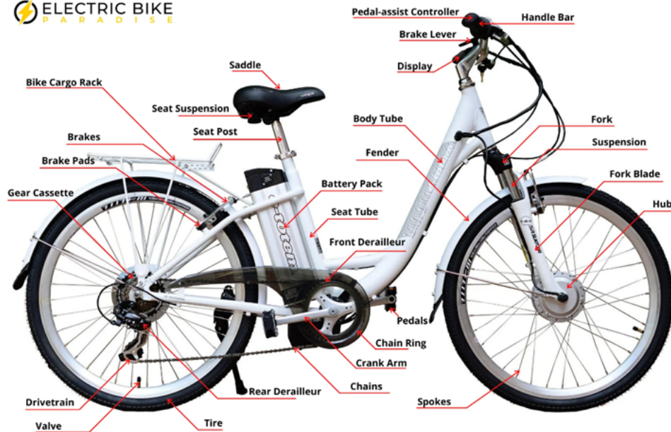
Figure 2-11: Anatomy of an e-bike (Electric Bike Paradise, 2019)
