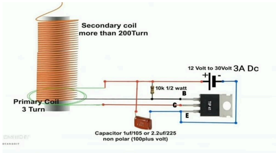
Fig 1: Schematic Diagram of Tesla Coil
