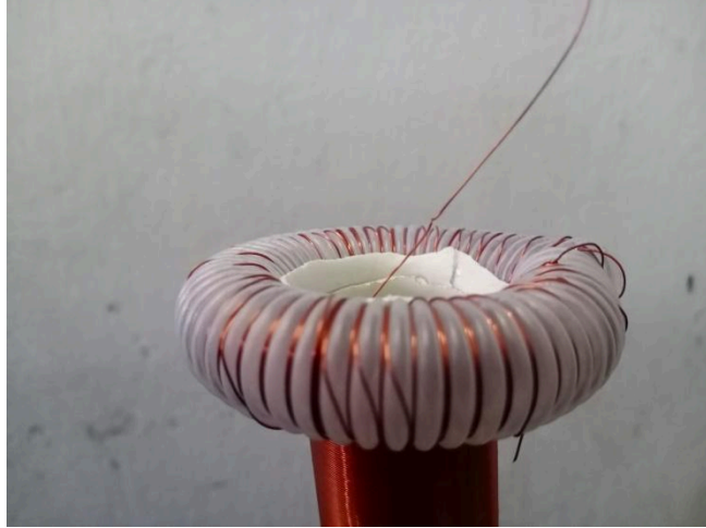
Fig 4: Secondary Coil
