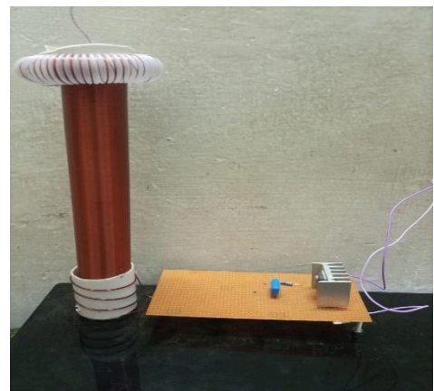
Fig 5: Complete Circuit
