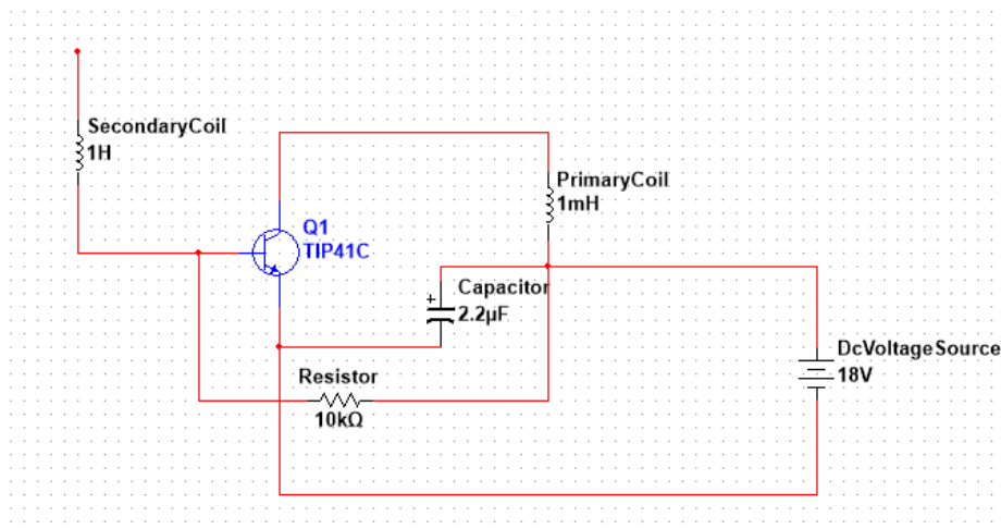
Fig 2: Circuit Diagram of Tesla Coil
