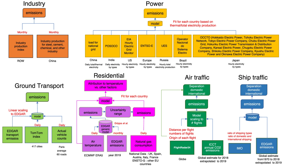
Fig 1. Overview of Carbon Monitor data production chain
