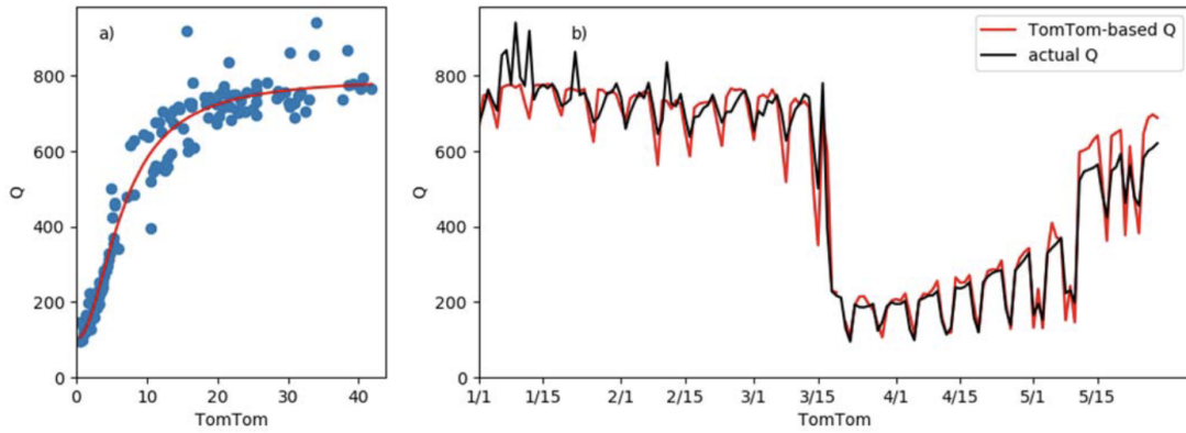
Fig 2 (a) Relationship between TomTom congestion level index and actual car counts (Q) for Paris. The sigmoid fit between and is given by the red line. (b) evaluation of the function during the period of the lock down in Paris.
